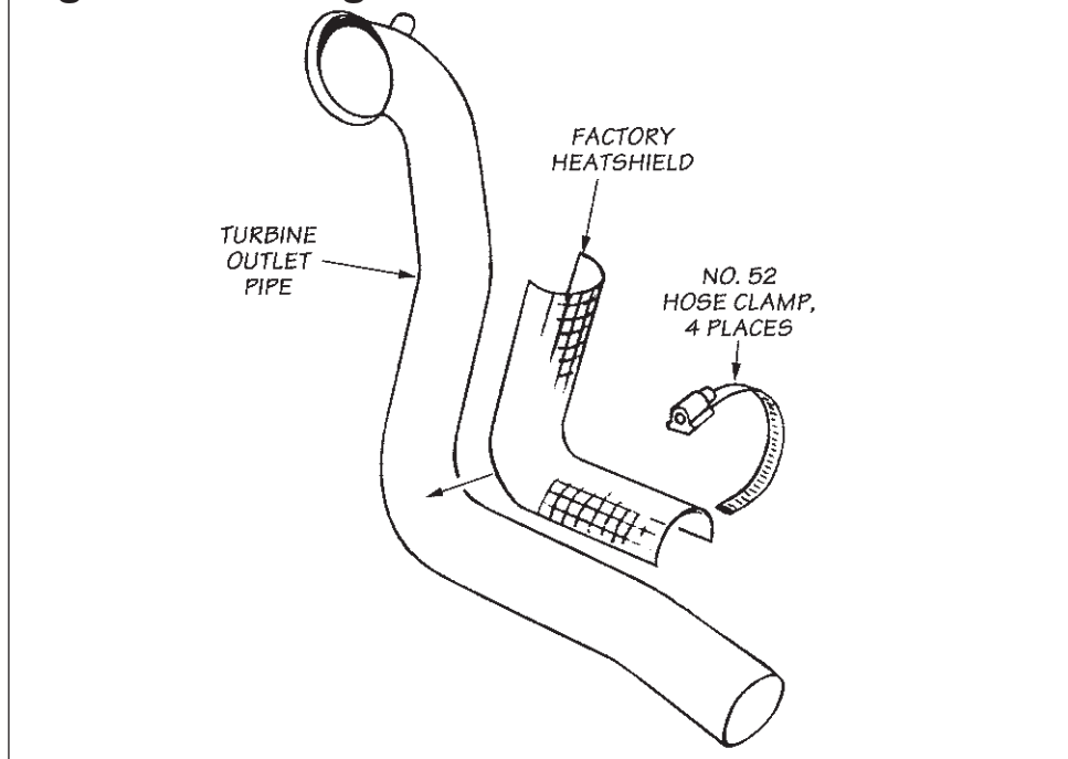
Figure 2- Securing Heat Shield
