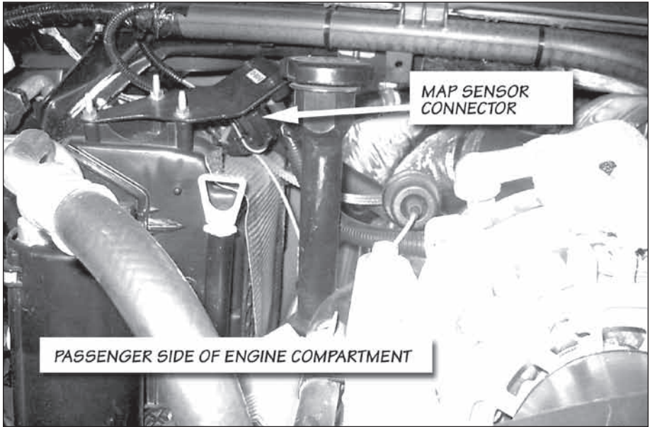
Figure 7: MAP sensor location
