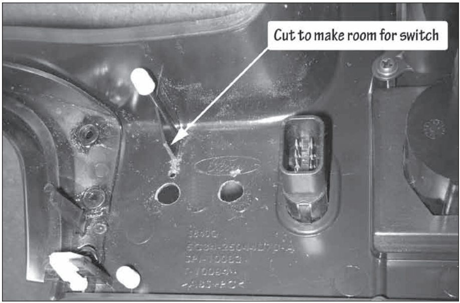
Figure 26: 05-07 Dash panel trimming
