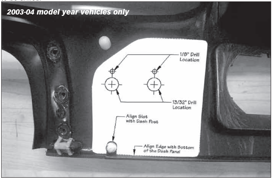
Figure 24: Template taped to back of dash on 2003-04 model year vehicle, ready to be drilled.
