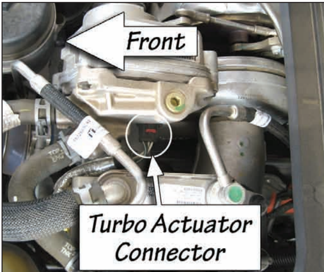
Figure 4: Turbo Actuator Connector
