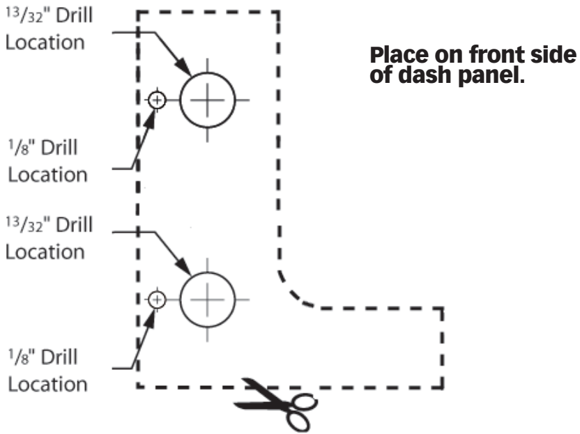
Figure 24 Template for locating the Banks Brake and Six-Gun switch on the dash panel
