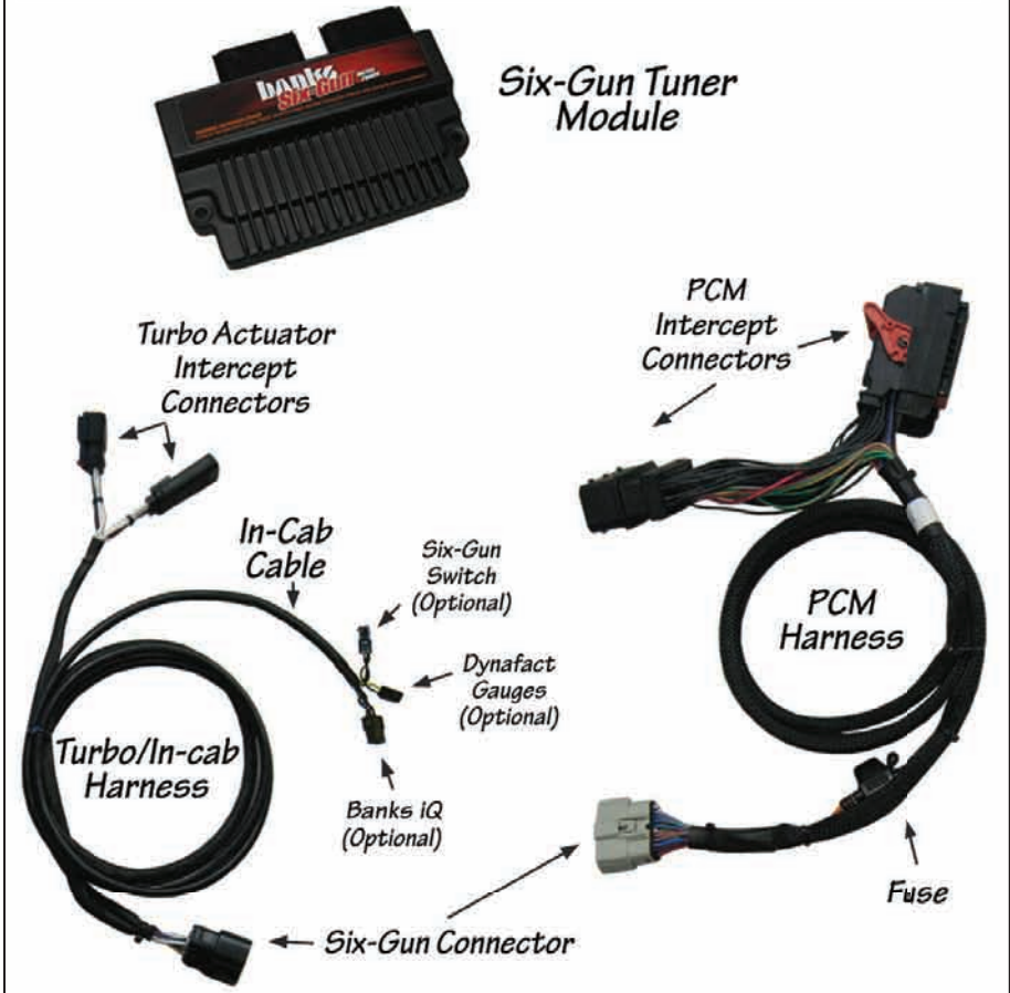
Figure 1: Banks Six-Gun and supplied wiring harness
