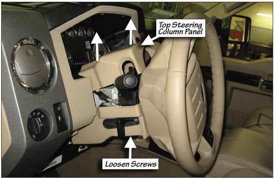
Figure 13 Remove top column panel cover
