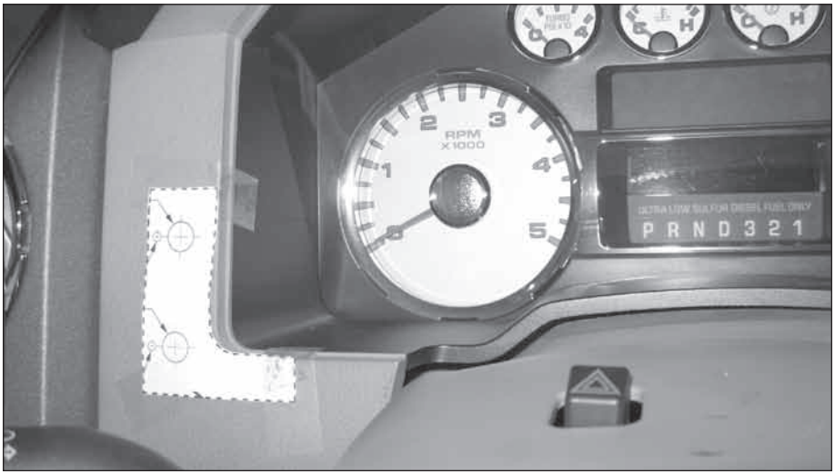
Figure 18 Template taped to front of instrument cluster
