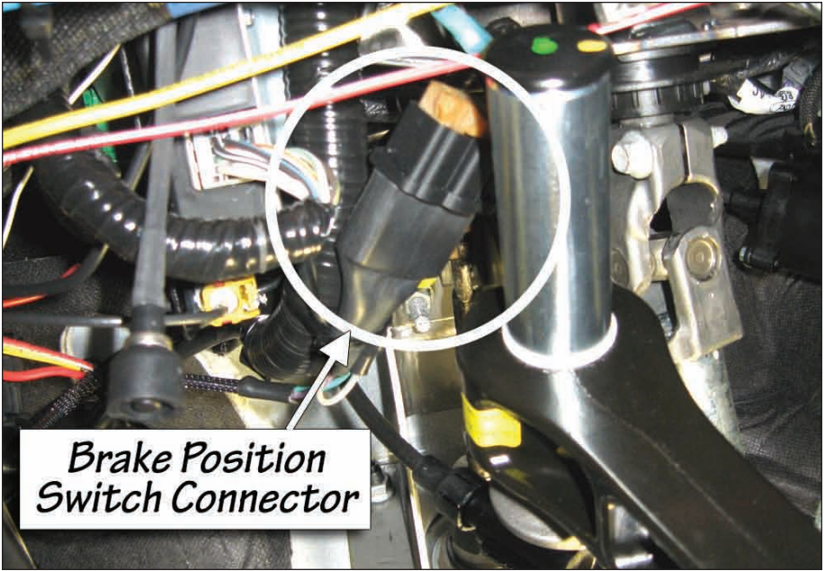
Figure 12 Brake Position Sensor location under dash
