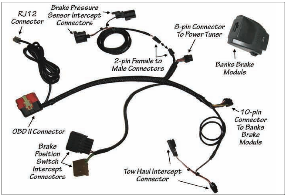
Figure 10 Banks Brake Wire Harness
