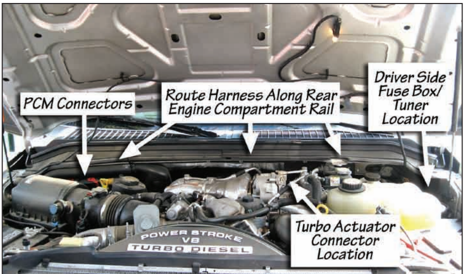
Figure 2: Six-Gun Harness routing
