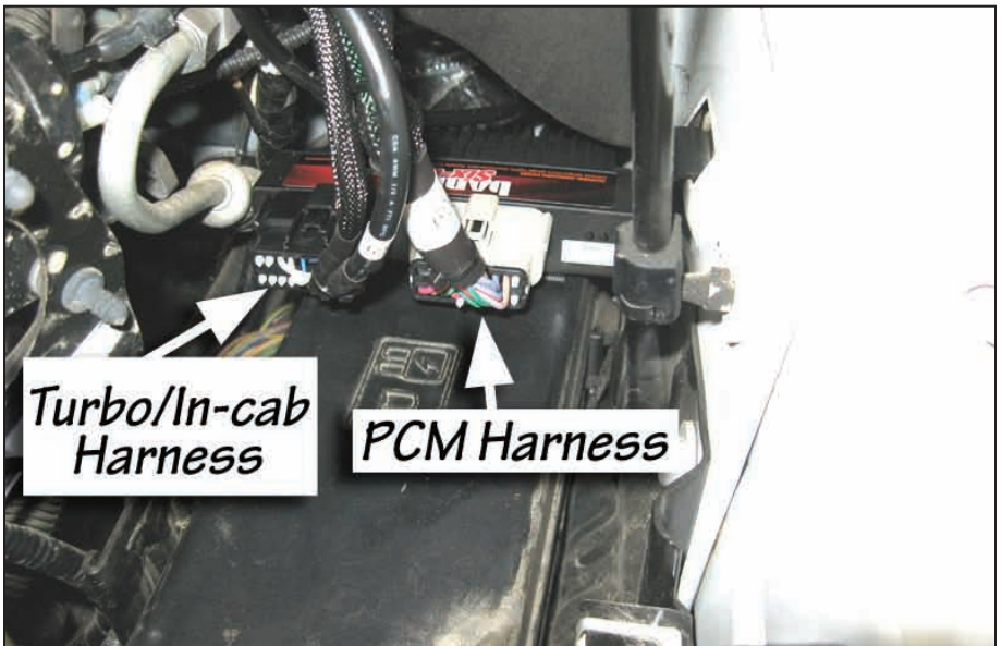
Figure 8 Mounting location of Six-Gun tuner to Fuse box, driver
