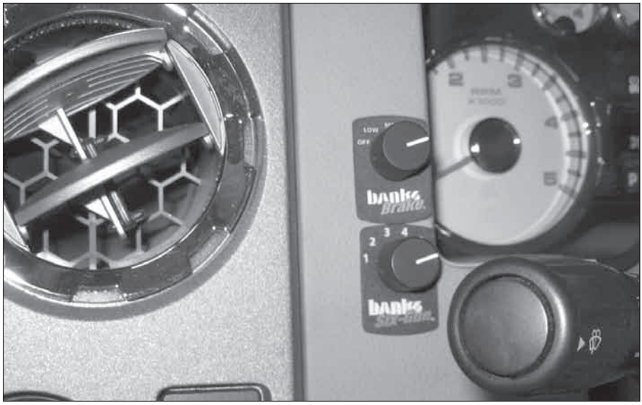
Figure 21 Finished installation of the Six-Gun/Banks Brake Switch
