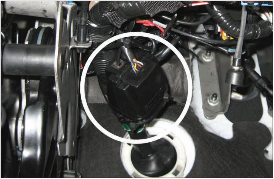
Figure 15 Banks Brake Module mounting location
